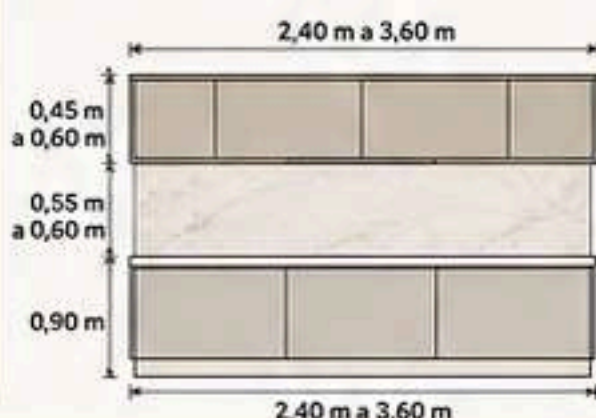
VISTA FRONTAL
